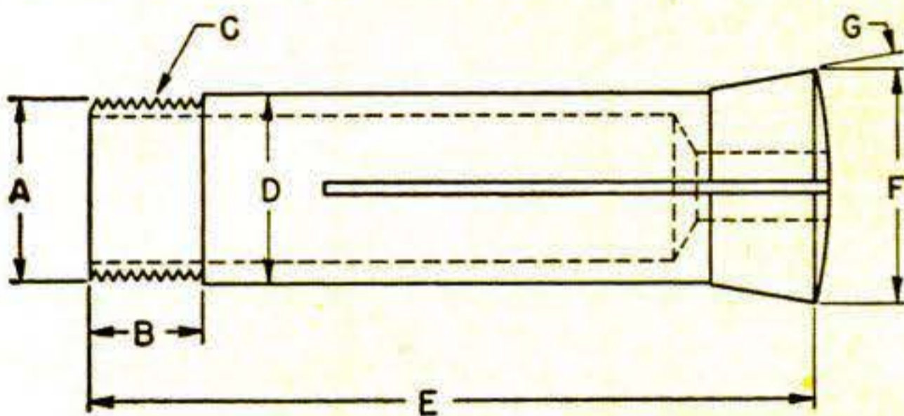
Specifications of Steel and Brass Collets
